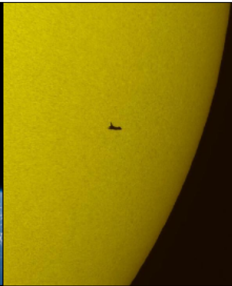
solar transit
