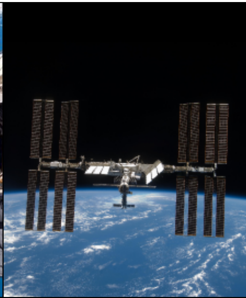
space station
