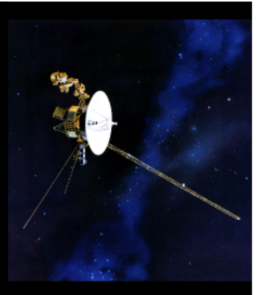
probe
