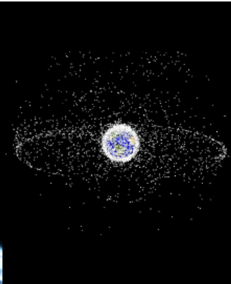
space junk
