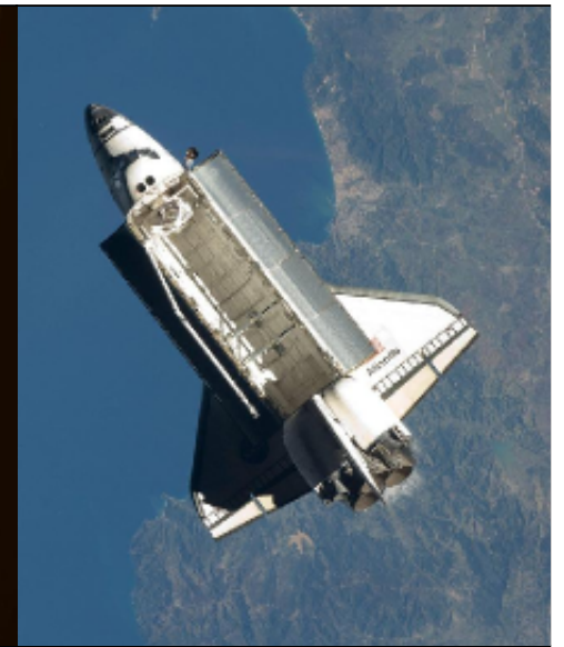
space shuttle
