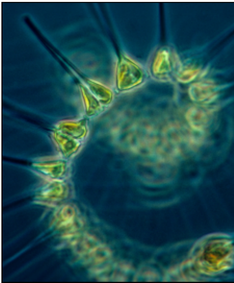
phytoplankton
