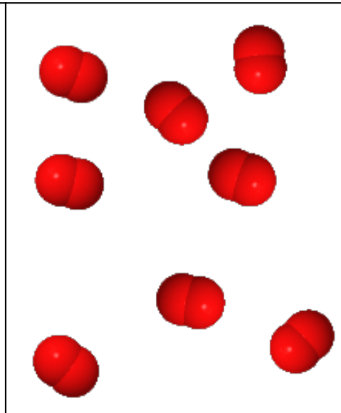
oxygen
