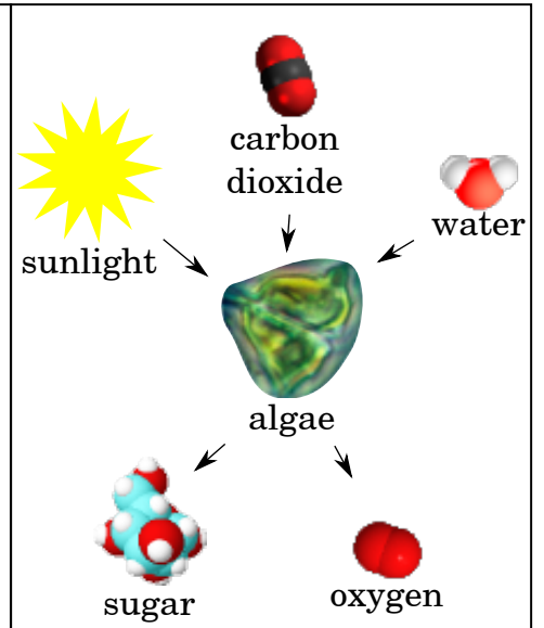
photosynthesis
