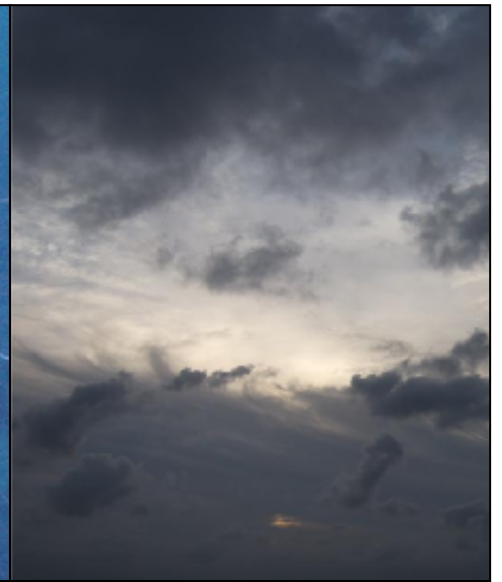
atmosphere
