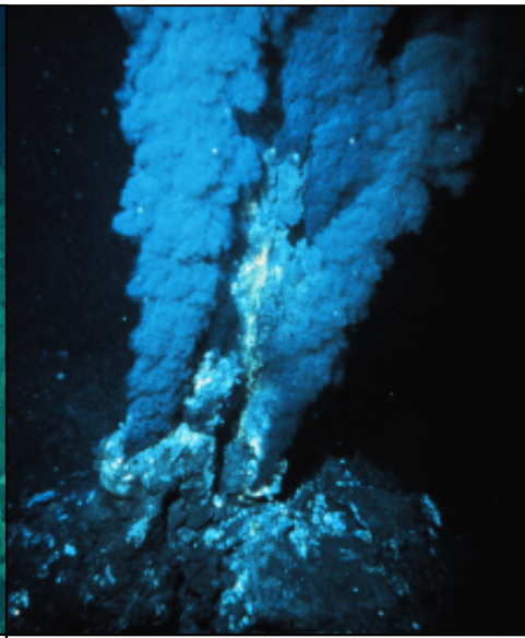
black smoker
