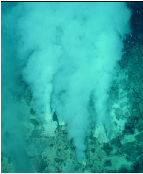
white smoker
