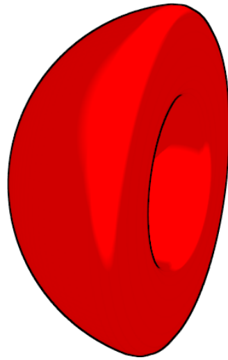
mantle
