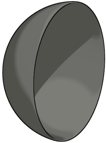
crust
